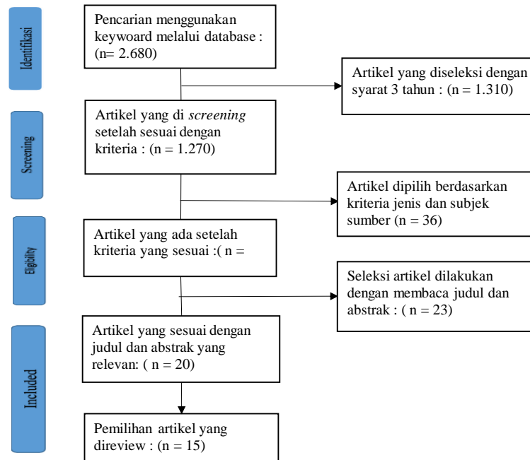
Gambar 1 : Prisma study flow diagram
