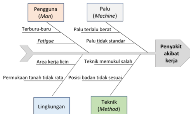
Gambar 3. Diagram Fishbone
