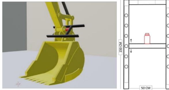
21 Gambar 2. Desain Special Tool
