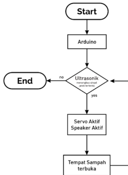
Gambar 2 Flowchart Rangkaian
