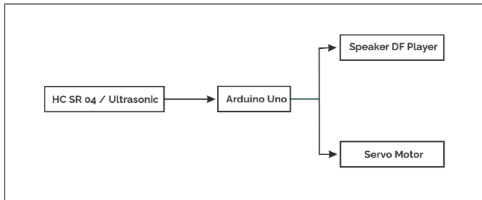
Gambar 1 Blok Diagram
